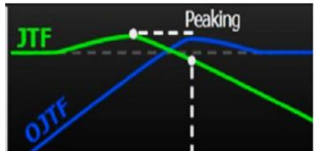
Figure 22. The M8040A provides a built-in- clock recovery option. You can choose between a first and second order PLL characteristic
